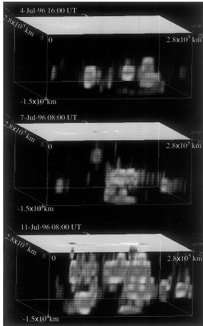
Fig. 16. Volume rendering of the sound-speed perturbation in the emerging active region NOAA 7879 on 4-Jul-96, 16:00 UT (top panel), 7-Jul-96, 8:00 (middle panel), and 11-Jul-96, 8:00 (bottom panel). The interior of the Sun is viewed from beneath. The panel on the top is a magnetogram showing the surface magnetic field of positive (white) and negative (black) polarities. The horizontal size of the box is approximately 280 Mm, the vertical size is 15 Mm. The perturbations of the sound speed which range from -1.5 to 1.5 km/s, are negative (dark grey) beneath the sunspots in the bottom panel, and positive (lighter grey) in other places (Electronic Annex available. See http://www.elsevier.nl/locate/cam ).
