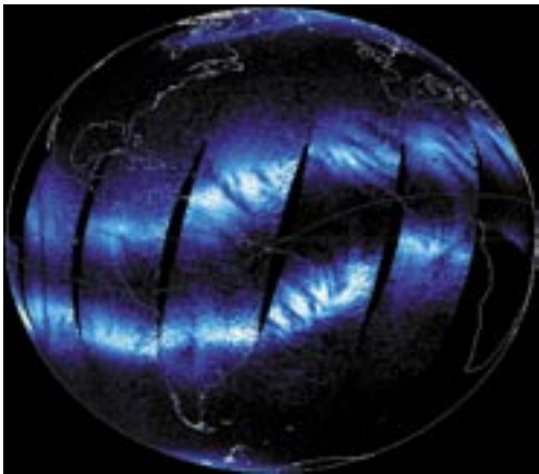
Image of electron density enhancements (equatorial arcs) in the Earth’s ionosphere. The transport of plasma away from the equator results in traveling densities enhancements and depletions in bands poleward of the equator. These exist during the daytime and most of the night and create enhanced media transmission errors in navigation and communication signals.
