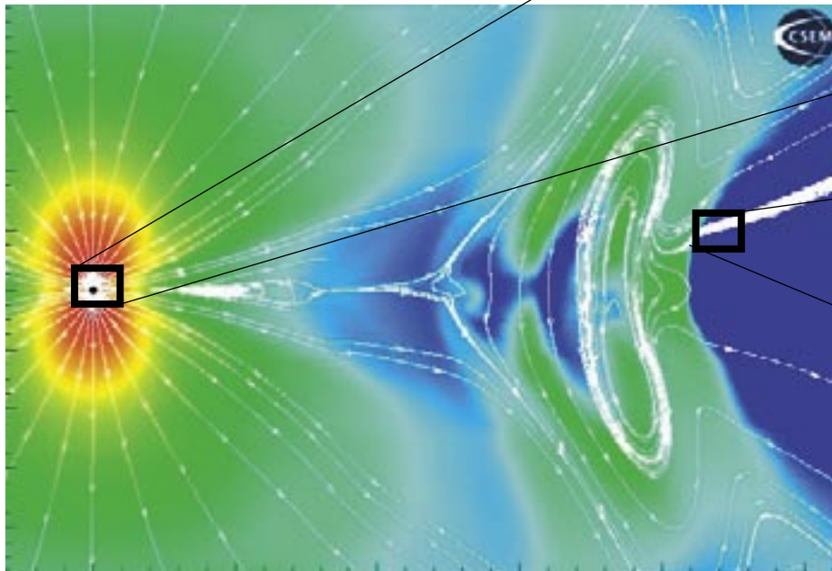
Several kinds of space plasma simulation models have been developed to provide a theoretical understanding of the flow of energy from the Sun through interplanetary space to the Earth's magnetosphere. This first frame illustrates the progression of a coronal mass ejection (CME). Shown are magnetic field lines (white) and magnetic field strength (low = blue to high = red) 20 hours into an event. The sun is the small black dot at the center of the red glow to the left. The CME is at the right riding on top of the expanding flow of the solar wind at speeds up to 2,000 kilometers per second.
