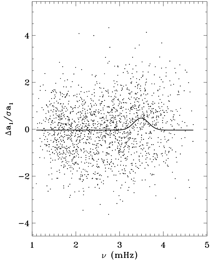
vector weighted
