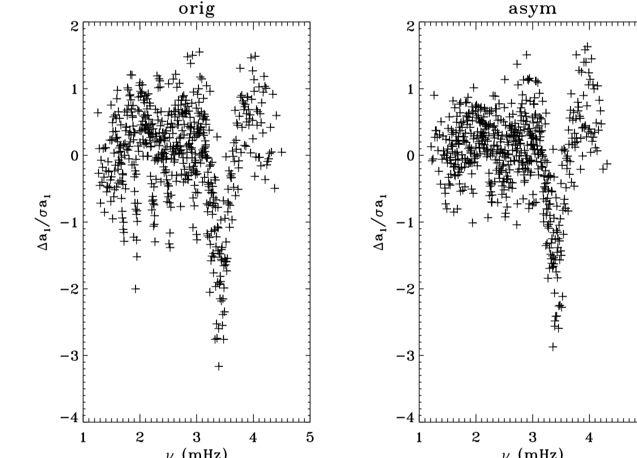
Figure 5: Normalized residuals of a_1 for the original analysis and after all corrections. These plots have been binned in frequency for clarity.
