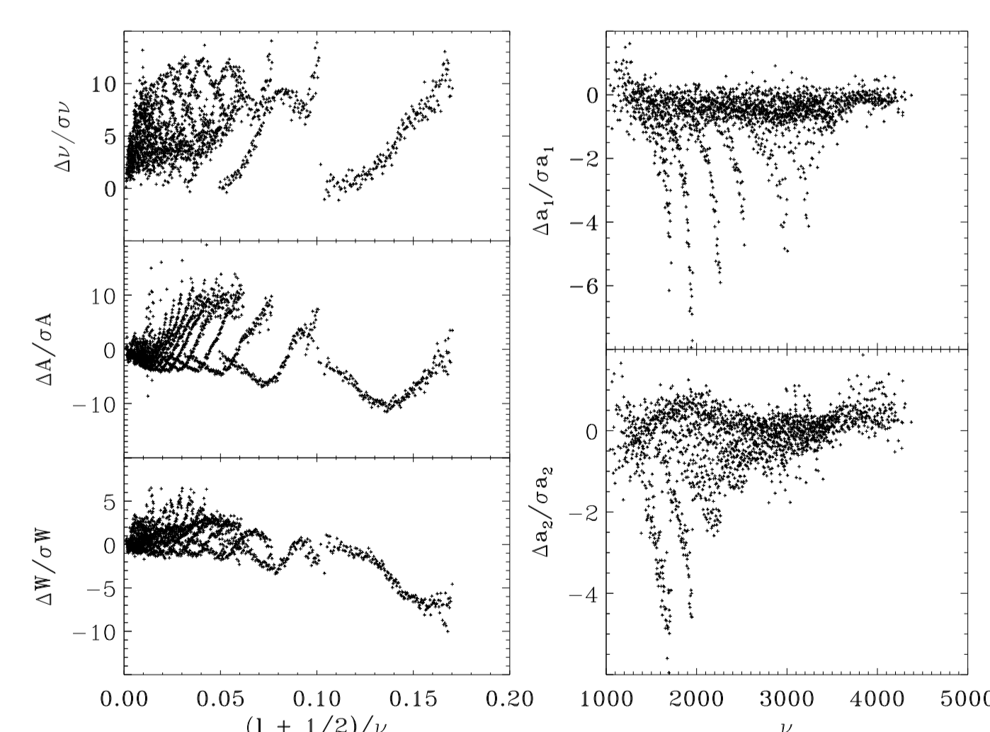
Figure 2: Comparison of original and final analyses for frequency, amplitude, linewidth, a_1 and a_2 .
