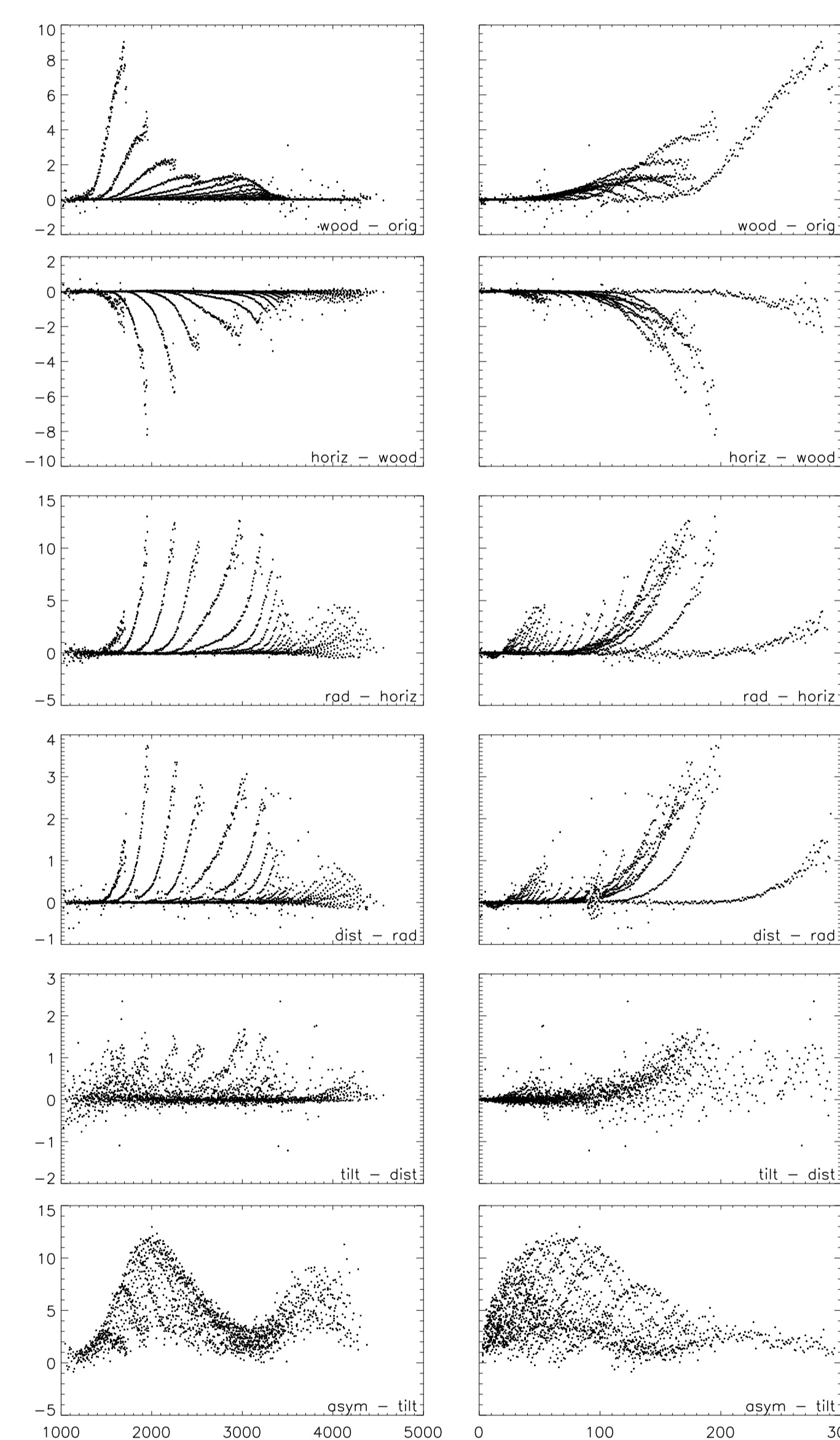
Figure 1: Frequency differences between selected analyses in units of standard deviation, on the left as a function of frequency in \mu\text{Hz} , on the right as a function of l .
