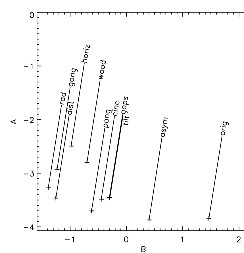
Figure 4: Phase diagram for frequency changes. Plus signs mark the initial point, straight lines indicate the change made by the Doppler correction. Note that one would expect the magnitude of "gong" to be lower than "gaps" because it averages over a longer time.
