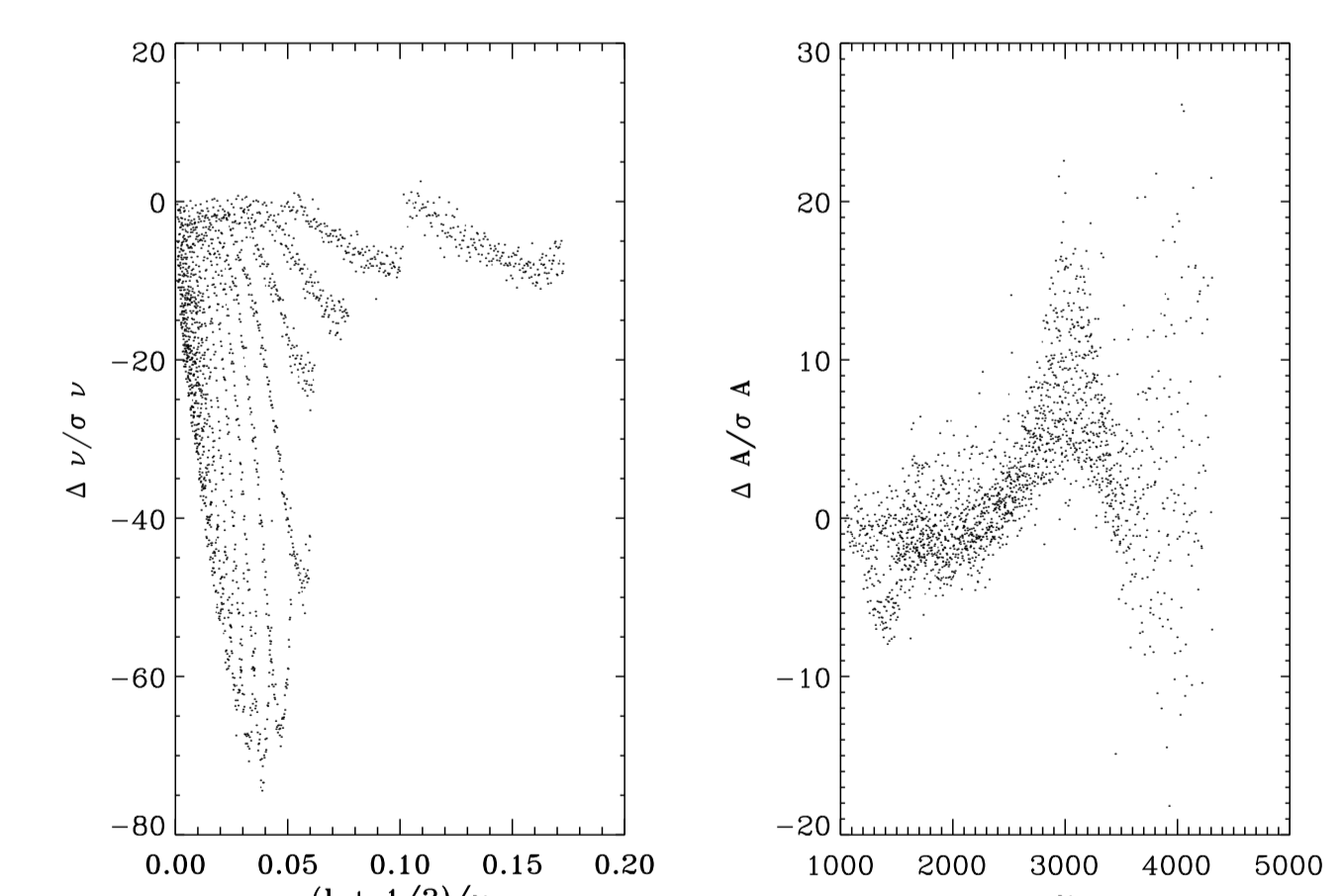
Figure 7: Results from an analysis of the first eight years of data with only the radius corrected, compared to the original analysis. Note that as we average over longer times, the error goes down.
