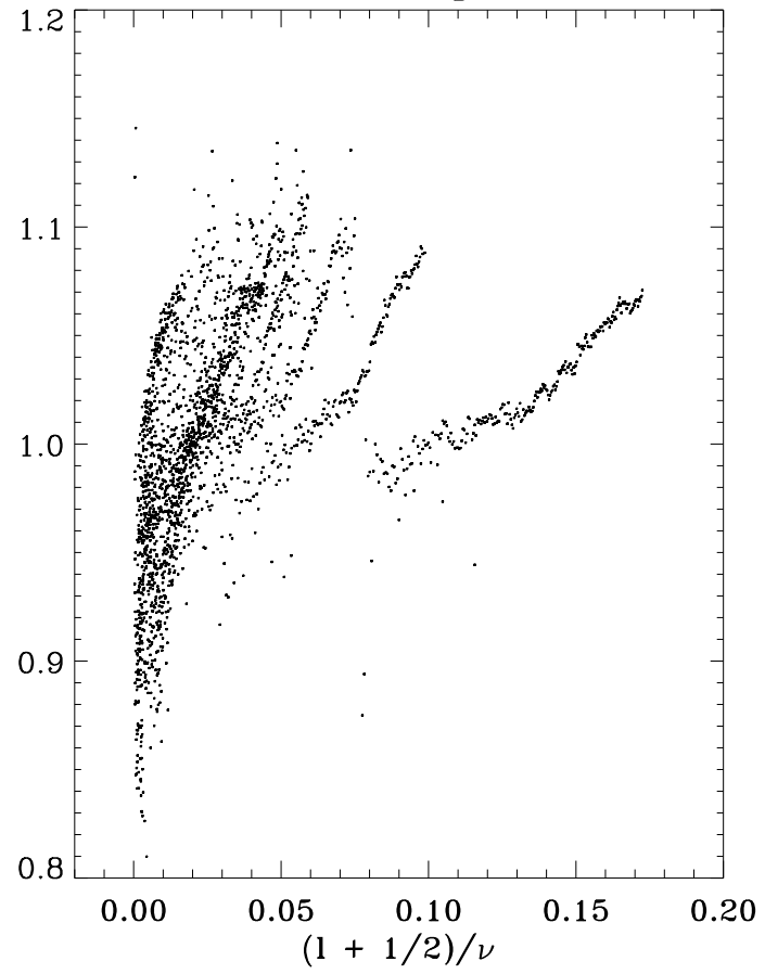
vector weighted
